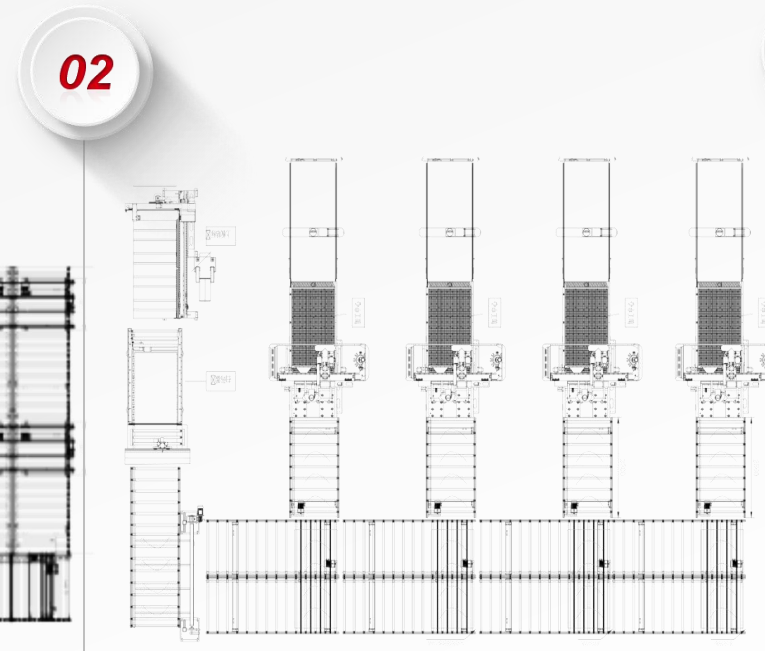
4 Sets Cnc Router Machine Line
